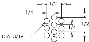
Perforated Screen Detail
