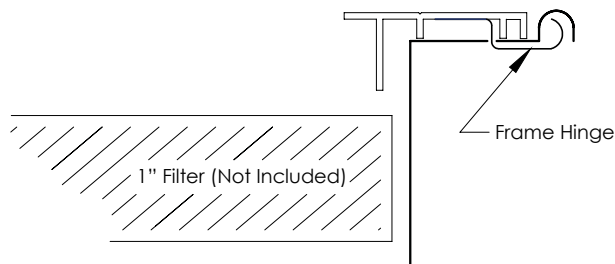
645FG1 Frame Detail
