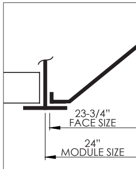
T-BAR MOUNT DETAIL
