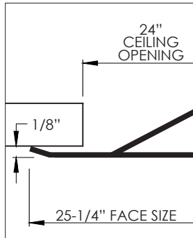
SURFACE MOUNT DETAIL
